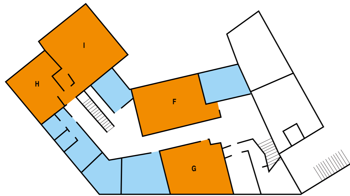
PIANO SEMINTERRATO
